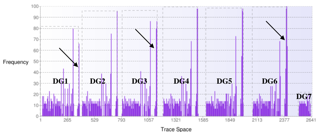
Figure 4.18. The result of applying the integrated scheme on Phase2
