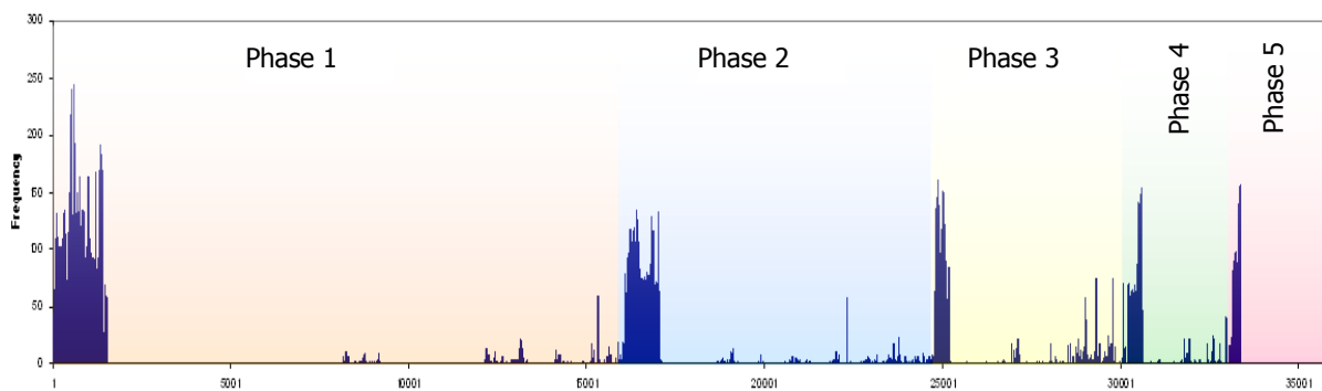
Figure 5.8. Detected phases for execution trace of ArgoUML
