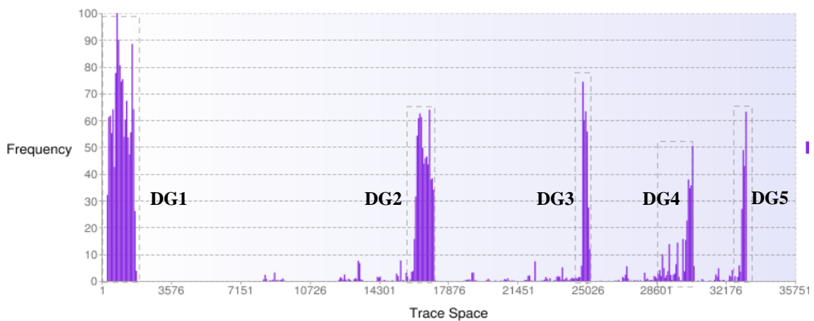
Figure 4.21. Dense groups formed on the rearranged trace of ArgoUML
