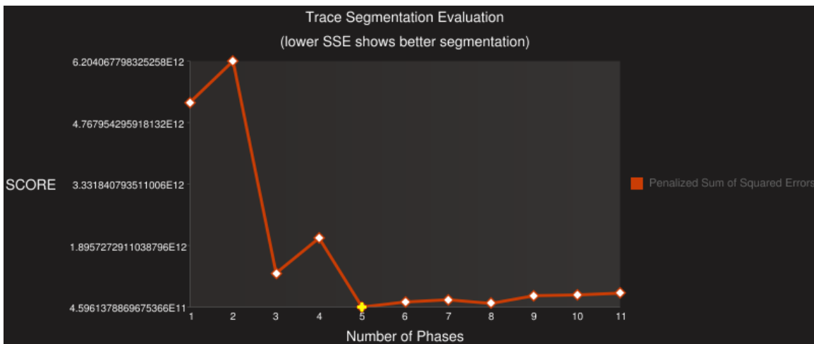
Figure 4.22. PSSE scores for different partitionings
