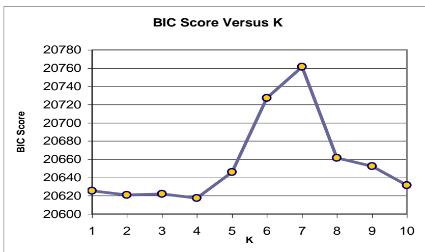
Figure 4.19. The BIC score for different partitionings of DG2, the partitioning with 7 clusters is the fittest
