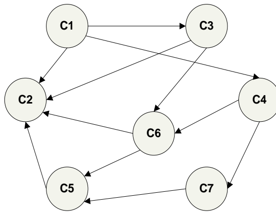
Figure 3.3. Example of a class dependency graph
