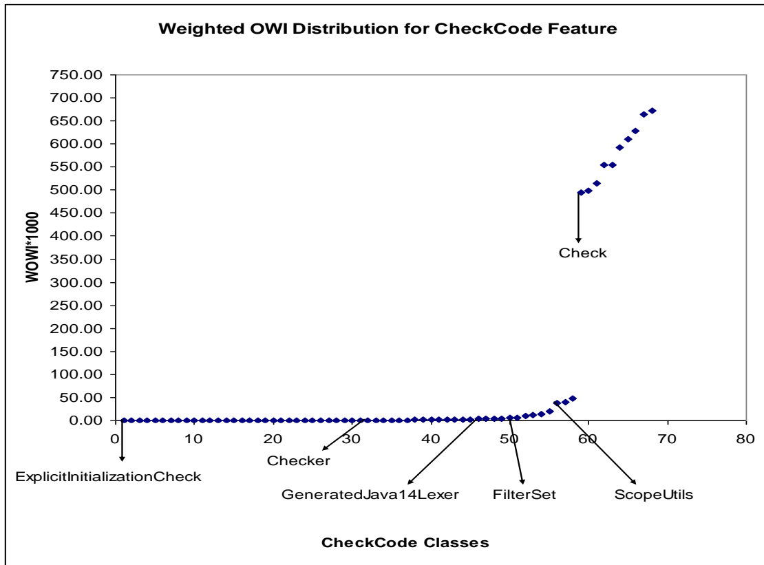
Figure 4.5. WOWI distribution for CheckCode feature.
